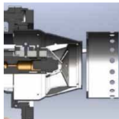
Combustion Head.
